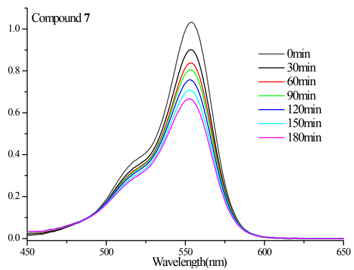
Fig. s6 photodegradation properties of compounds 4 , 5 and 7 .
