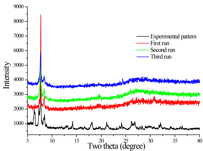
Fig. s5 experimental and X-ray powder diffraction patterns after three runs of repeated experiments of compound 7
