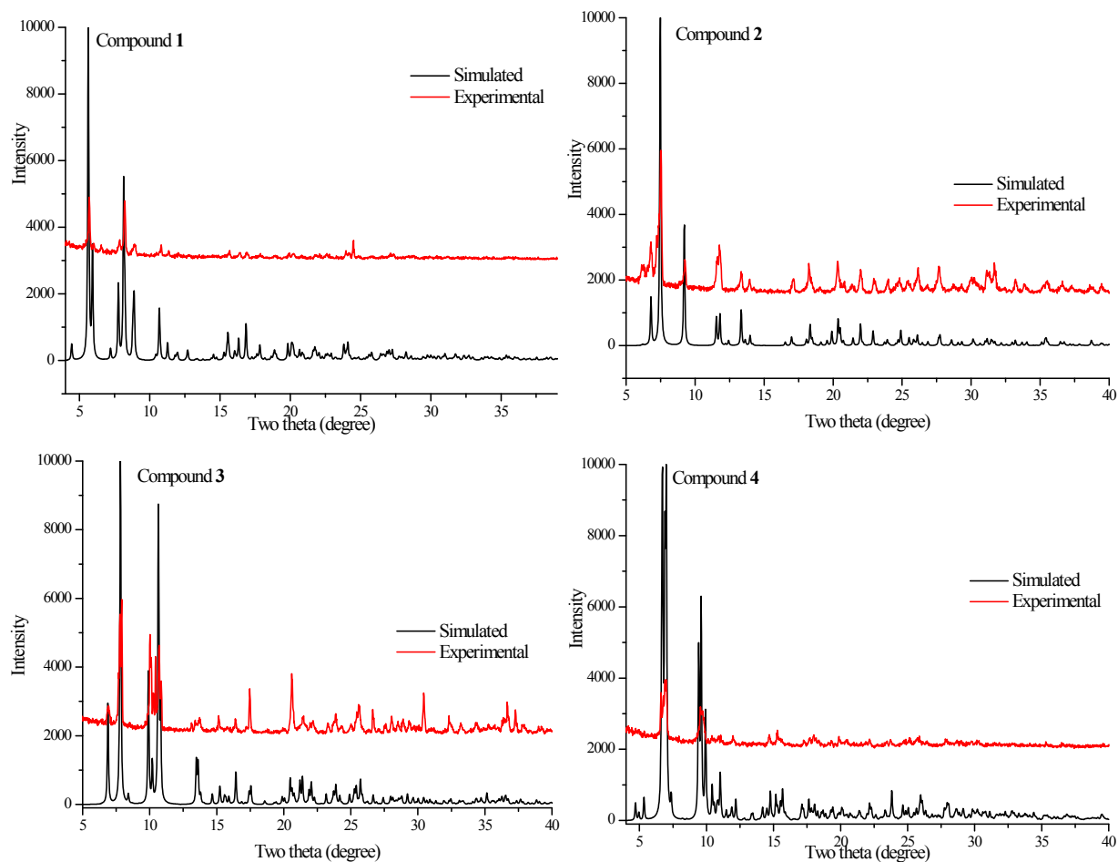
Fig. s2 simulated and experimental XRD patterns of compounds 1-4.
