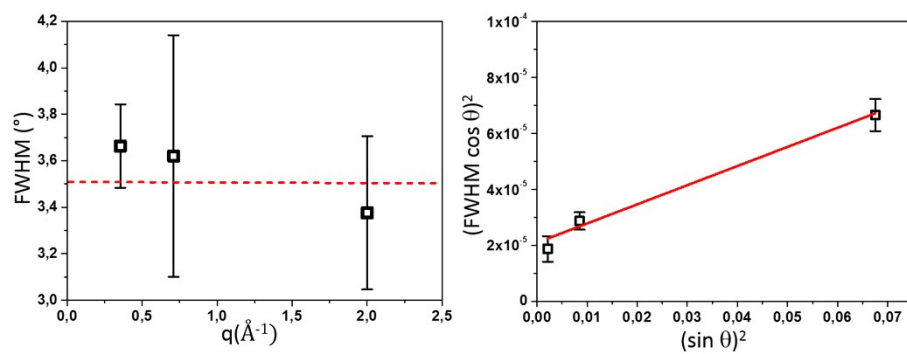
Figure I. (a) mosaicity determination from FWHM and (\beta \cos \theta)^2 variation as a function of (\sin \theta)^2 for grain size determination (b) through Williamson-Hall relation.
