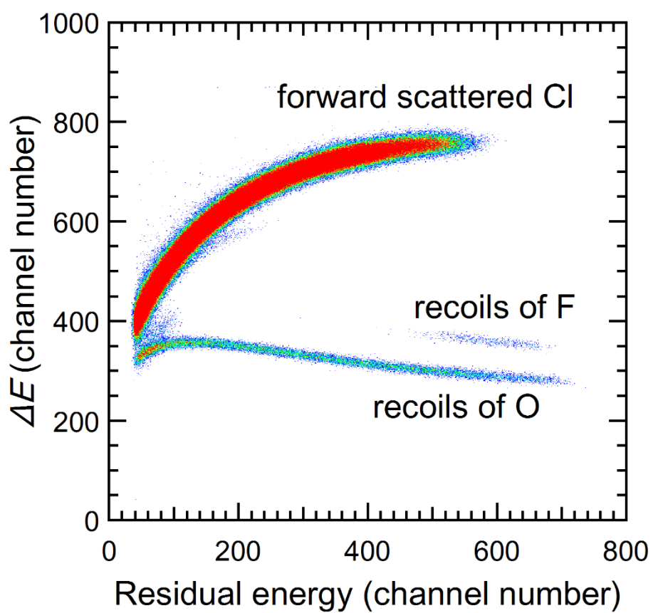
Supplementary figure S2. \Delta E - E ERDA histogram taken on the \text{Sr}_2\text{RuO}_4 film fluorinated at 240 °C. Apart from the intense Cl signal, the recoil signals of O and F were clearly observed.
