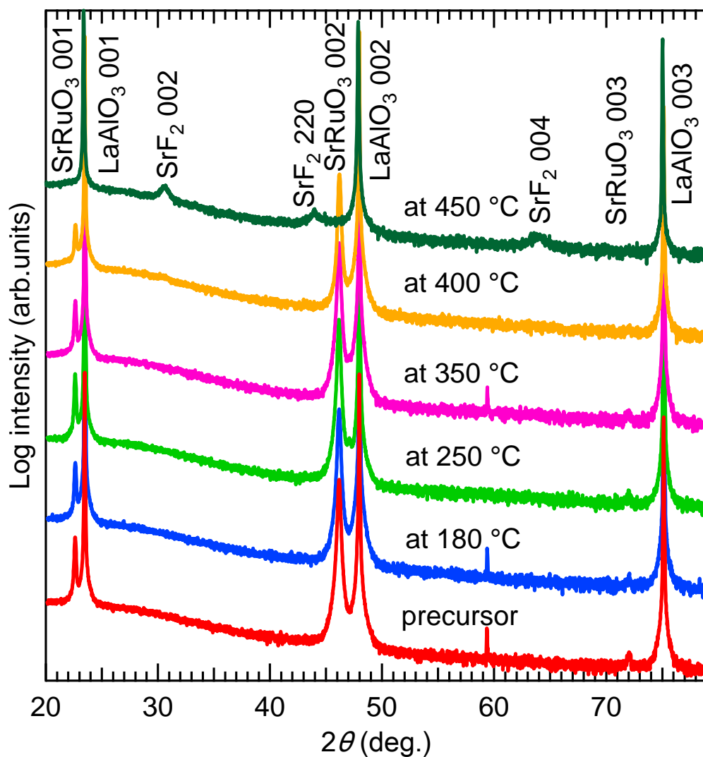
Supplementary figure S1. 2\theta - \theta X-ray diffraction patterns of the SrRuO 3 precursor and the PVDF treated films at 180-450 °C on LaAlO 3 (001) substrates.
