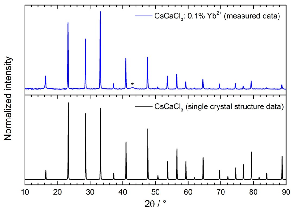
Figure S1. Measured XRD pattern of \text{CsCaCl}_3 : 0.1% \text{Yb}^{2+} (blue) compared to the diffraction pattern based on single crystal structure data (based on reference 54 in the main article). The black asterisk marks a reflection from the silicon grease used for the sample preparation.
