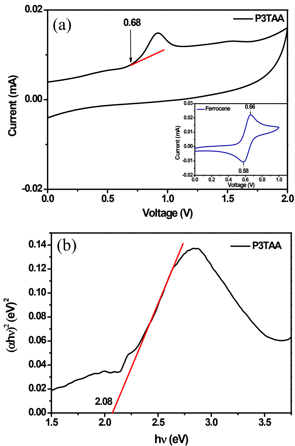
Figure S2: (a) Current-voltage curve obtained from cyclic voltammetry for P3TAA, (b) Tauc's plot of P3TAA
