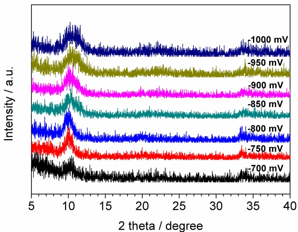
Figure S1. X-ray diffraction patterns of films deposited at different potentials.
