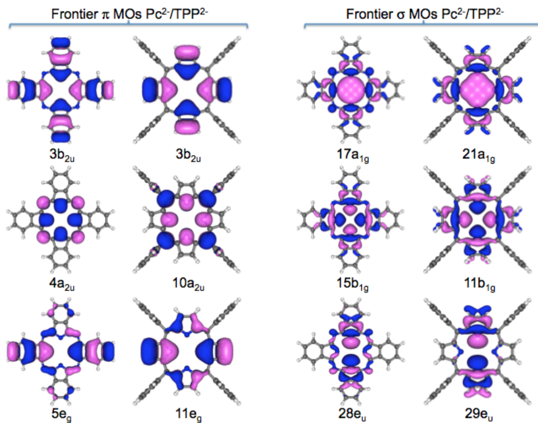
Figure S1. 3D contour plots of the N^{Py} -based Pc^{2-} and TPP^{2-} frontier \pi and \sigma MOs. Displayed isosurfaces correspond to \pm 0.02 e^{1/2} \text{ \AA}^{-3/2} values
