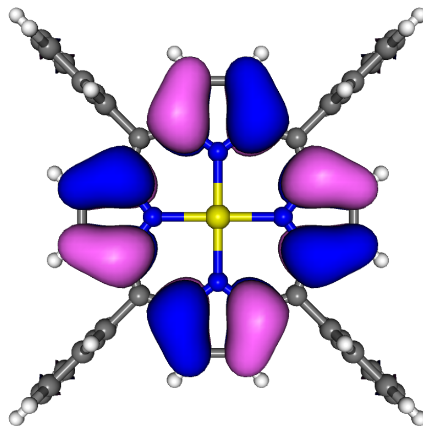
CuTPP
