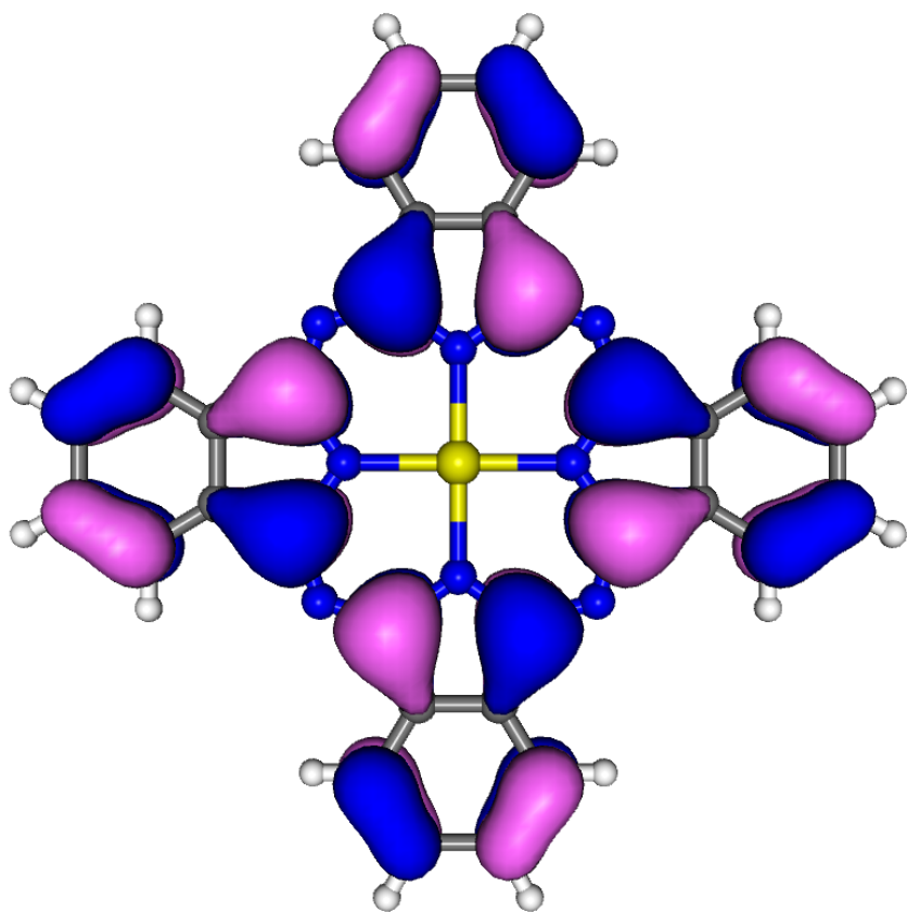
CuPc
