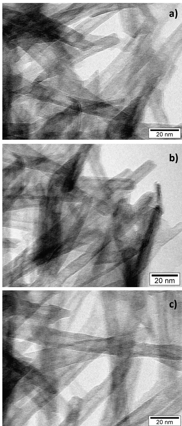
Fig. S1 – HRTEM images of the Co(5%)-TNT (a), Co(1%)-TNT (b) and TNT/Co(5%) (c) modified samples.
