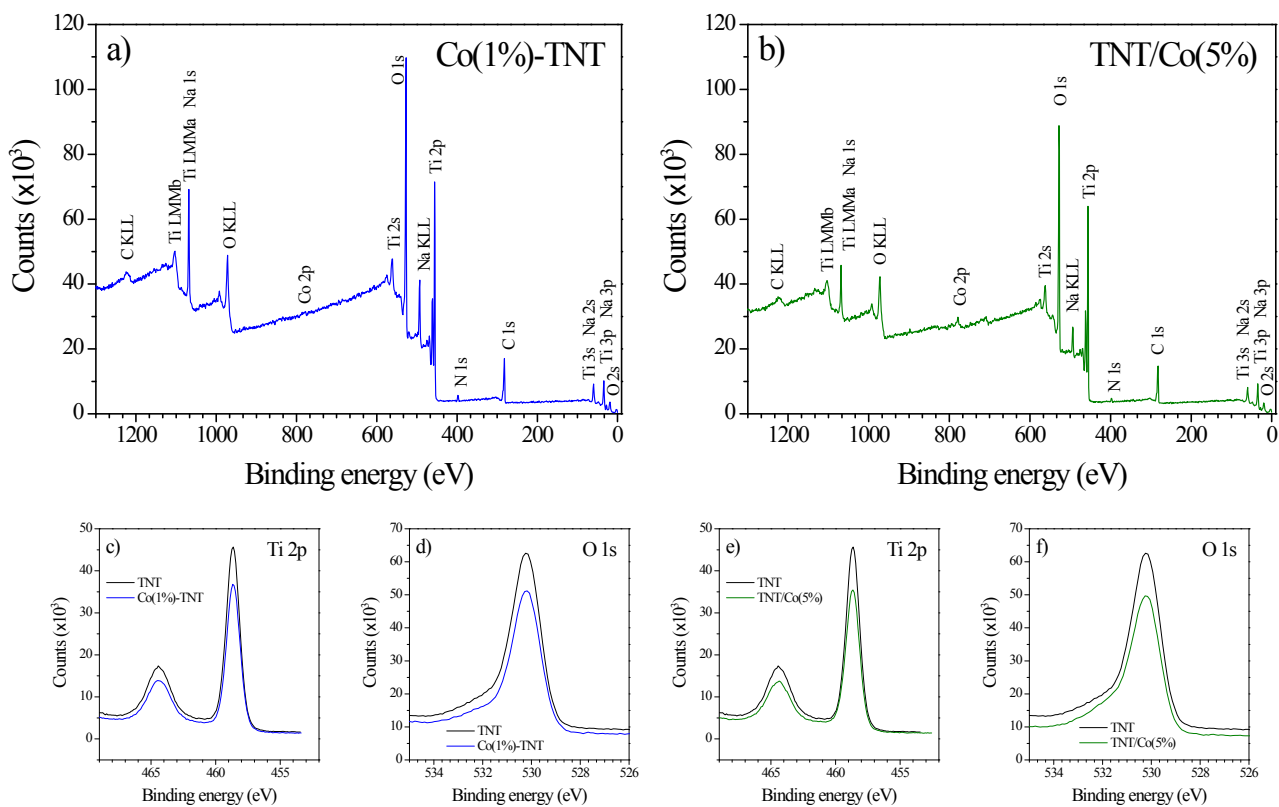
Fig. S4 - XPS survey spectra of the Co(1%)-TNT (a) and TNT/Co(5%) (b) samples. XPS high resolution spectra of the Ti 2p (c,e), O 1s (d,f) regions.
