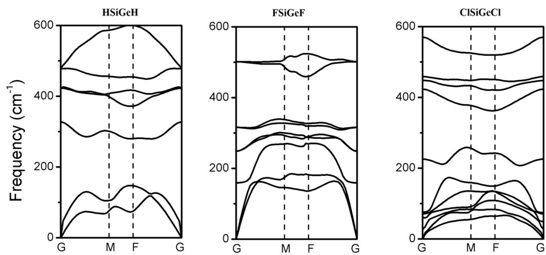
Fig.2S. The calculated phonon band dispersions of XSiGeX NSs, where X are H, F or Cl.
