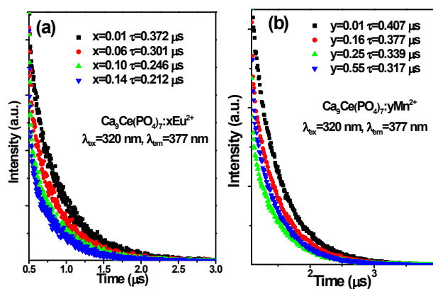
Figure S1 Photoluminescence decay curves of \text{Ce}^{3+} in \text{CCPO}:x\text{Eu}^{2+} and \text{CCPO}:y\text{Mn}^{2+} phosphors.
