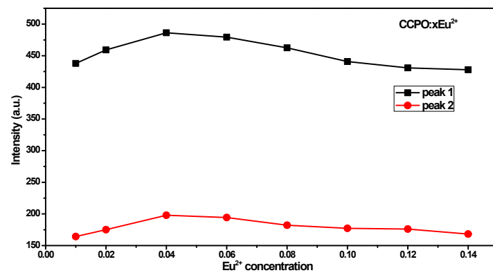
Figure S2 Intensity variation of the two sub-peaks of Eu 2+ in CCPO:xEu 2+ phosphors.
