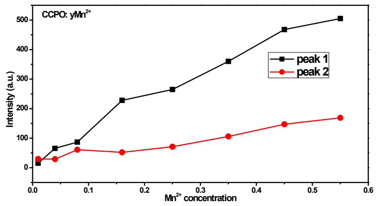
Figure S3 Intensity variation of the two sub-peaks of Mn 2+ in CCPO:yMn 2+ phosphors.
