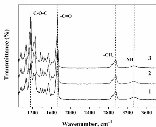
Fig. S1. FT-IR spectra of the non-oriented TPUU films after 2 weeks (curve 1), 30 month (curve 2) and 60 month (curve 3) of storage.
