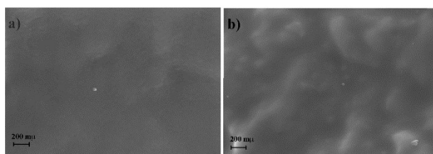
Fig. S2. SEM images of the non-oriented TPUU films after 2 weeks (a) and 60 month (b) of storage.
