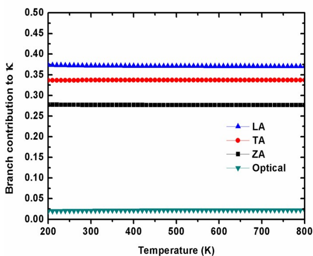
Fig. 1. Temperature dependence of branch contribution to lattice thermal conductivity.
