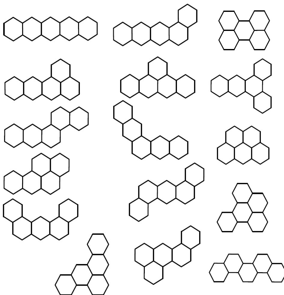
Figure S1. Accepted structures for the five-ring configuration.
