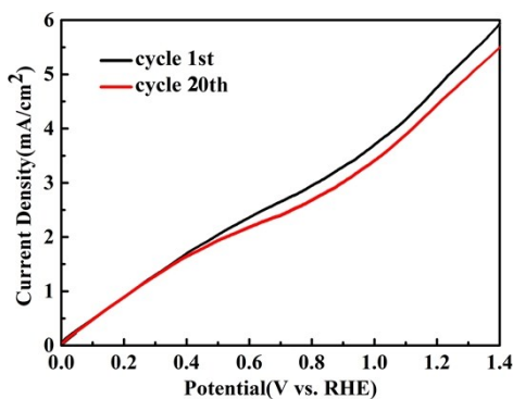
Fig.S1 Linear sweep voltammograms of the \text{TiO}_2/\text{Cu}_2\text{O} obtained with 120 sec deposition
