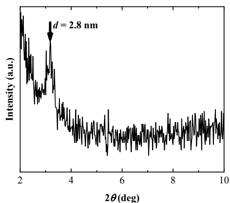
Fig. S2. XRD pattern of the LbL thin solid film with CoNS/TMPyP/CoNS sequence.
