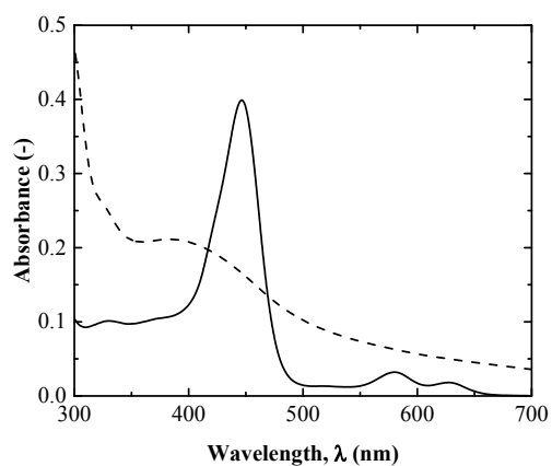
Fig. S1. UV-Vis absorption spectra of CoNS colloidal aqueous suspension (broken line) and TMPyP aqueous solution (solid line).
