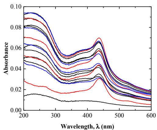
Fig. S3. UV-Vis absorption spectra of LbL thin solid film obtained after each operation (black lines: CoNS, red lines: TMPyP, and blue lines: MV).
