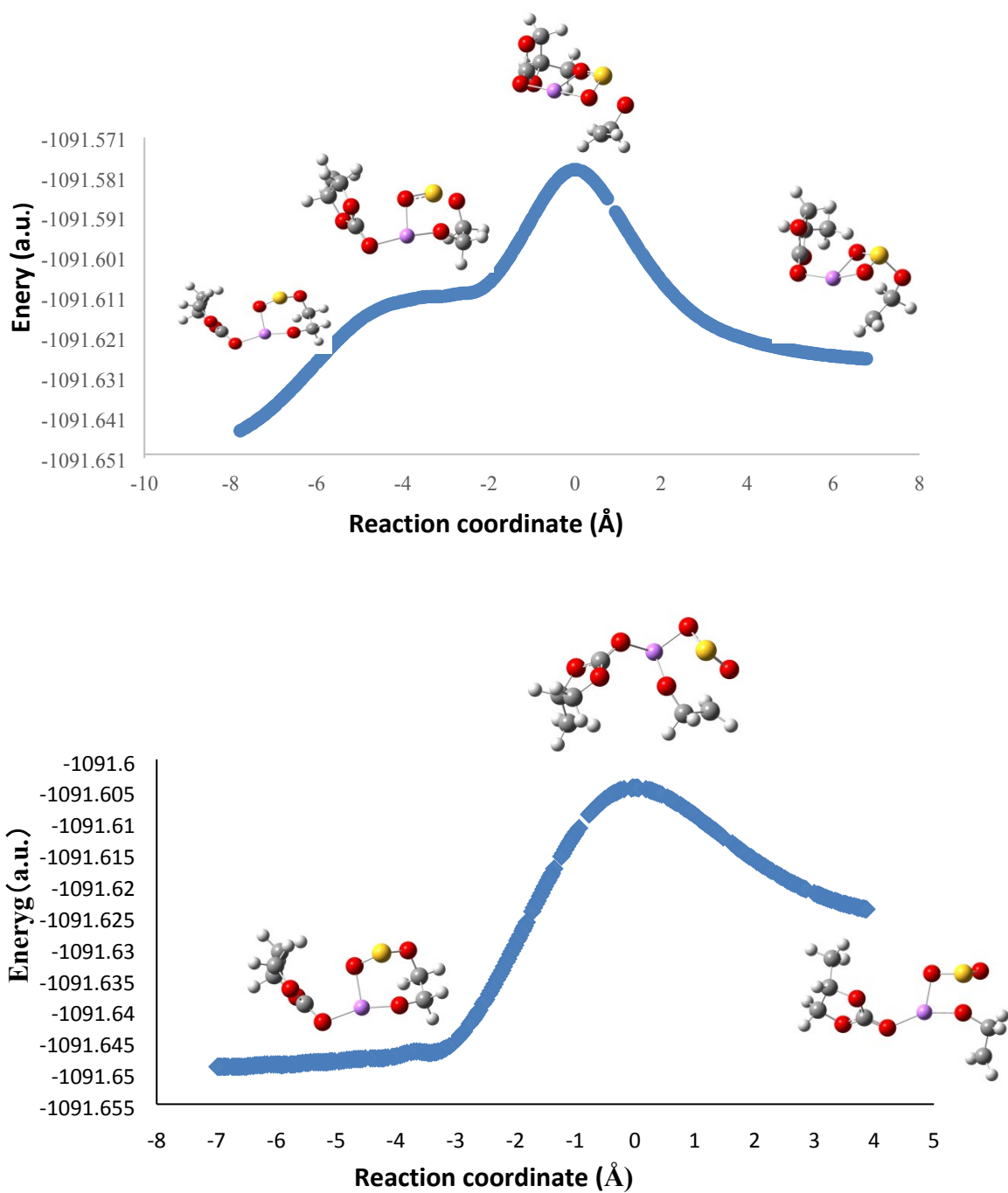
Figure S1. IRC calculations for the transition states 5 (top) and 7 (bottom).
