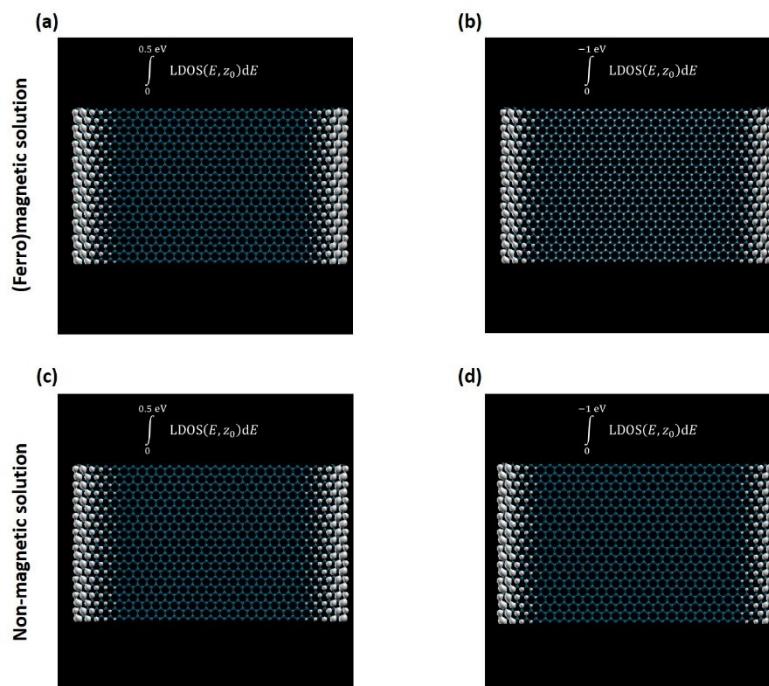
Supplementary Figure 1. Spatial distribution of (integrated) density of states for graphene ribbons with a_{21} type of the armchair edges. (a,b) Distribution of local density of states for ferromagnetic state; the integration is performed for states between Fermi level and 0.5 eV (a) and between Fermi level and -1.0 eV (b). (c,d) Same for the non-magnetic state.
