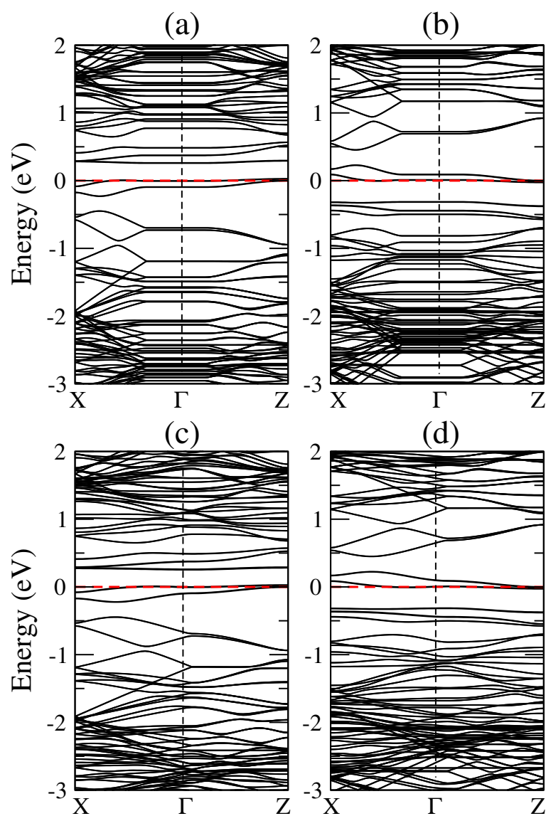
Figure 1: Electronic band structure for the B_3N_6 and B_6N_3 defects. Panels (a) and (b) refer to the enlarged unit cell while (c) and (d) refer to the LYP functional.
