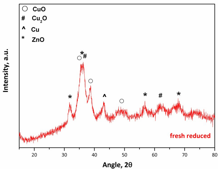
Fig. S1 : XRD pattern of the fresh reduced Cu:Zn:Al catalyst
