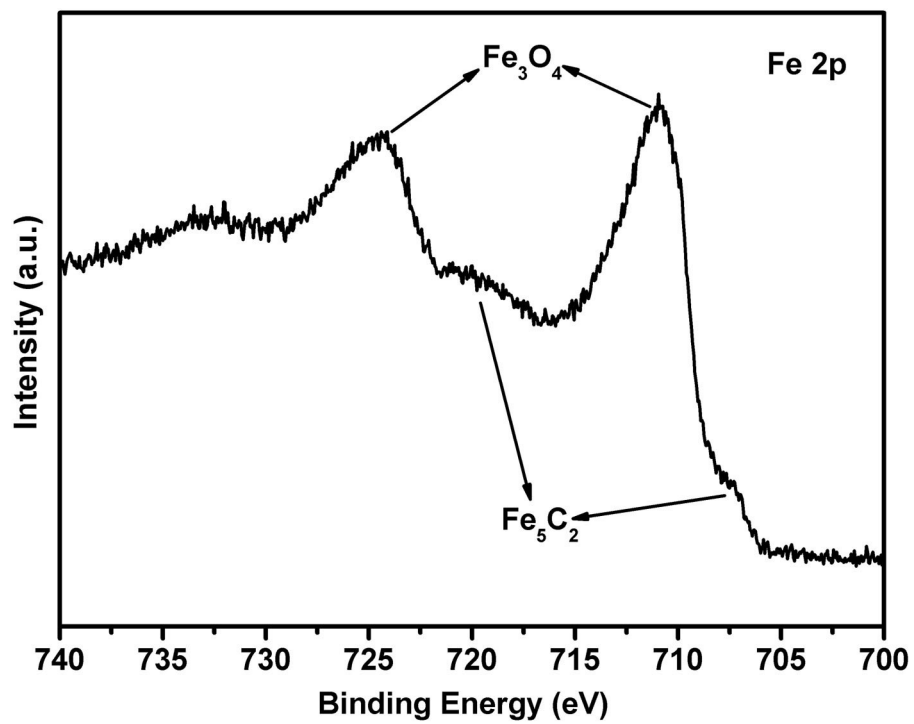
Fig. S4 Fe 2p XPS spectra of the used nanotube catalysts.
