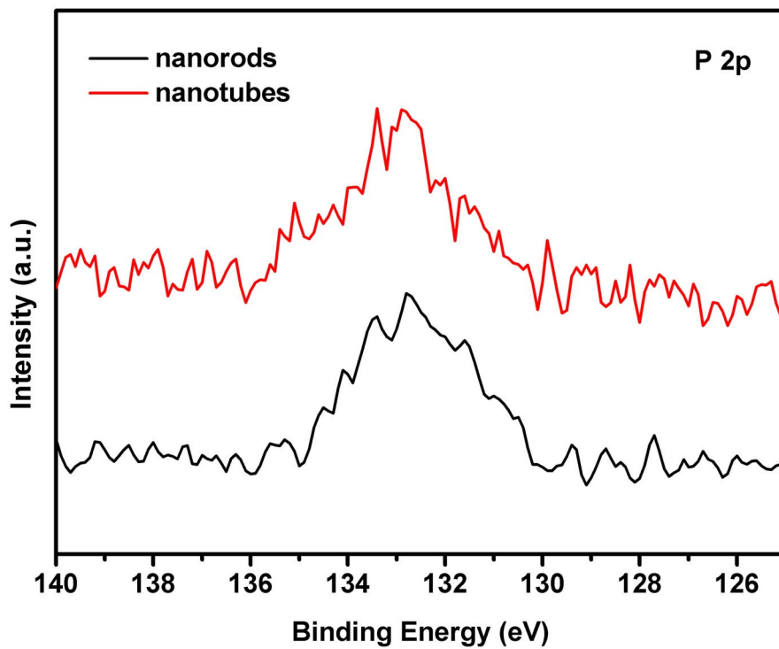
Fig. S3 P 2p XPS spectra of the 1D Fe 2 O 3 nanocatalysts.
