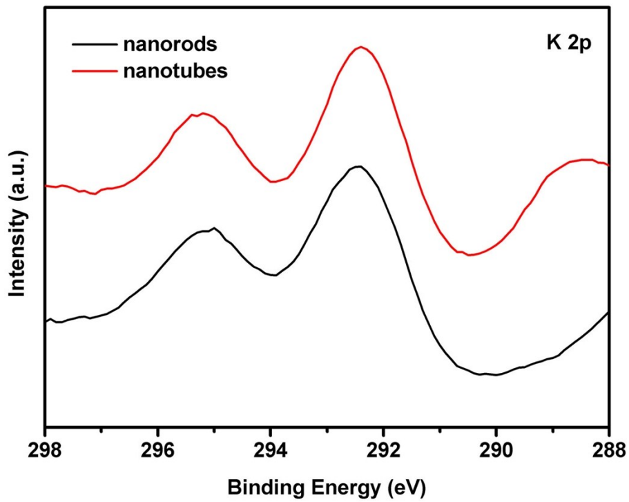
Fig. S2 K 2p XPS spectra of the 1D Fe 2 O 3 nanocatalysts.
