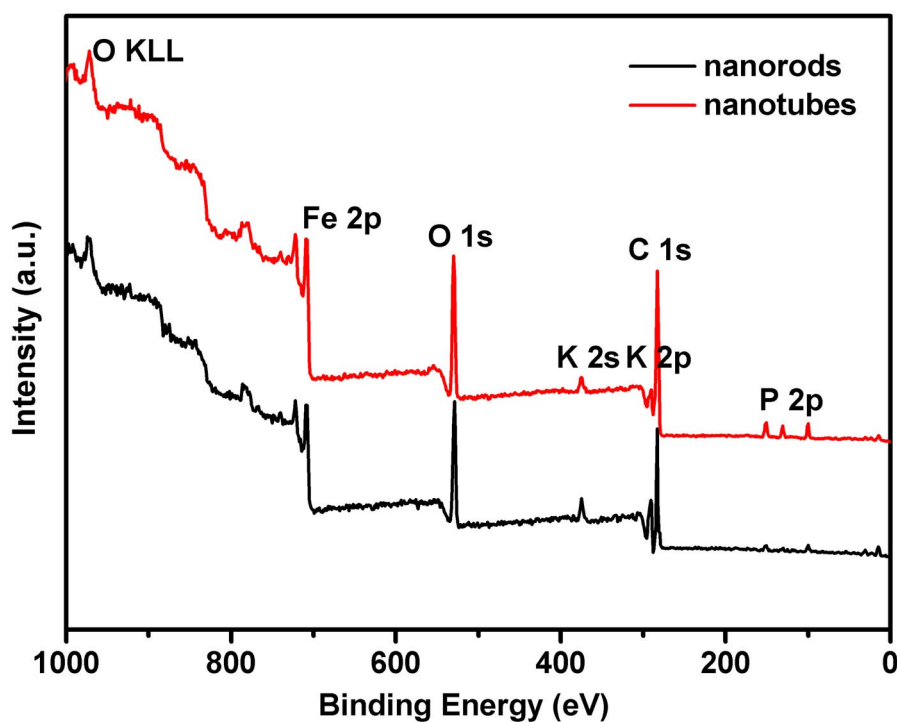
Fig. S1 XPS survey spectra of the 1D Fe 2 O 3 nanocatalysts.
