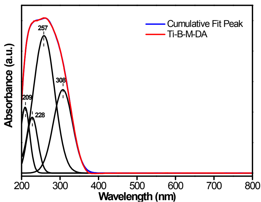
Figure S1. UV-vis spectra of Ti-B-DA and Ti-B-M-DA with their fit decomposition curves.
