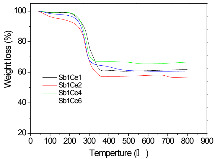
Figure S1. Thermogravimetric analysis of Sb1Cex catalysts.
