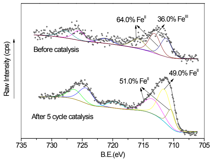
Fig. S2 XPS spectra of MIL-53(Fe)-2 before and after catalytic reaction.
