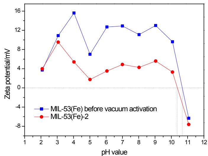
Fig. S1 Zeta potential of the as-prepared catalysts at different pH values.
