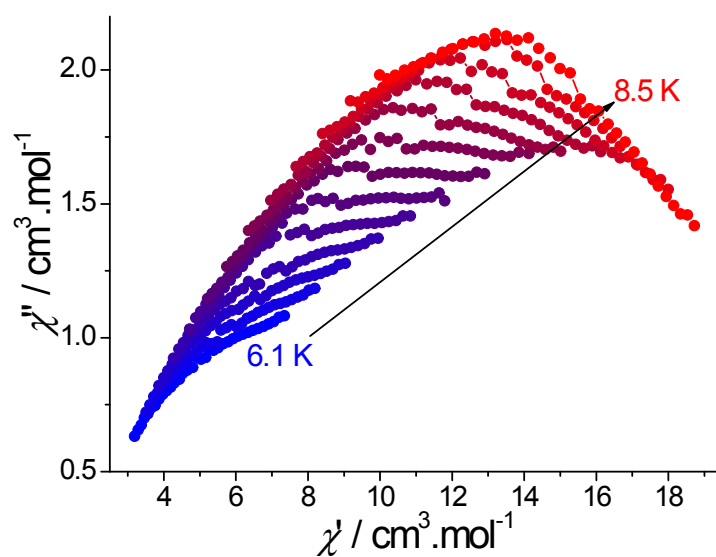
Figure S2. Cole-Cole plots for 1 .
