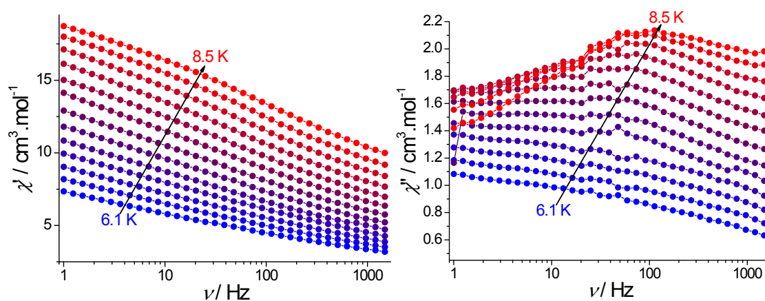
Figure S1. Frequency dependence of the in-phase (left) and out-of-phase susceptibilities (right) under a zero-dc field for 1 .
