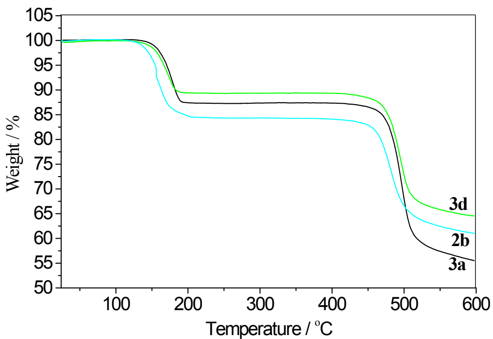
Fig. S7 Thermogravimetric analyses curves of compounds 2b , 3a and 3d .
