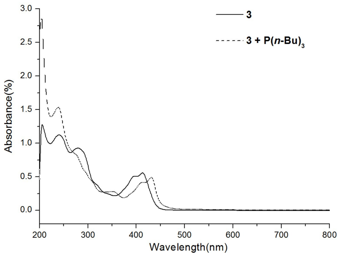
Figure S6. I UV-Vis absorption of complex 3 with Bu 3 P.
