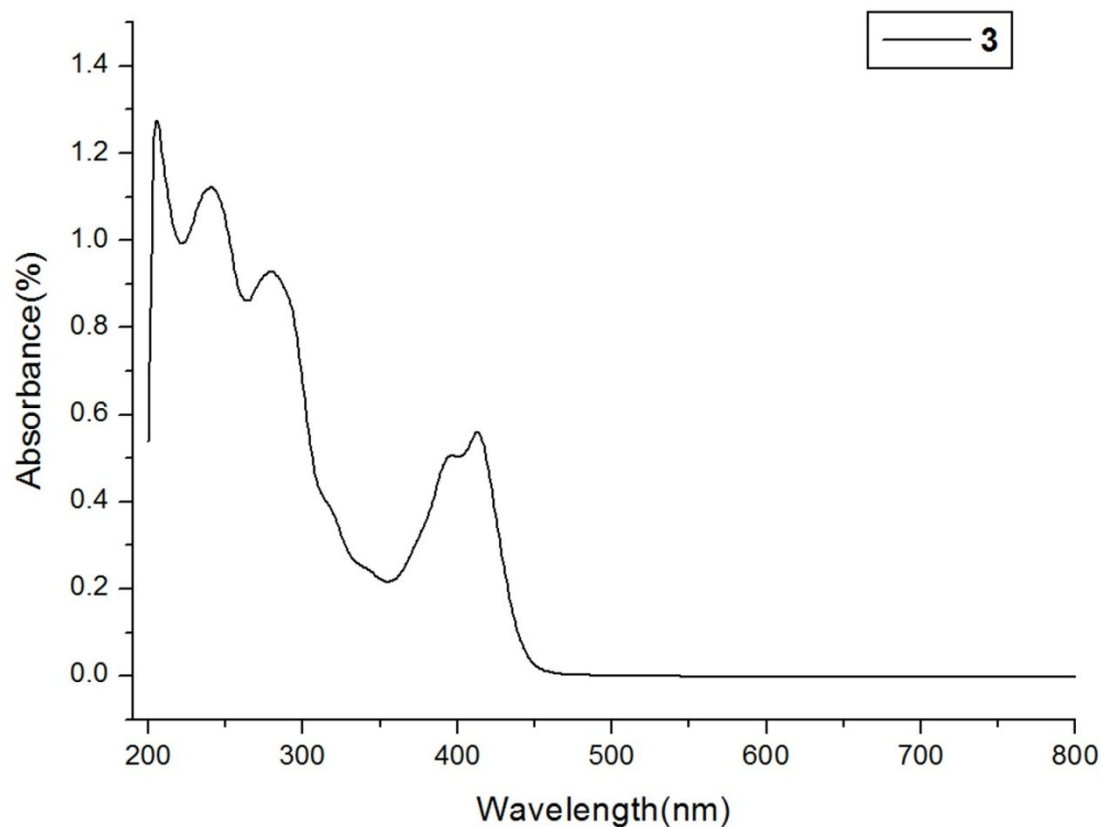
Figure S3. UV-Vis absorption of complex 3.
