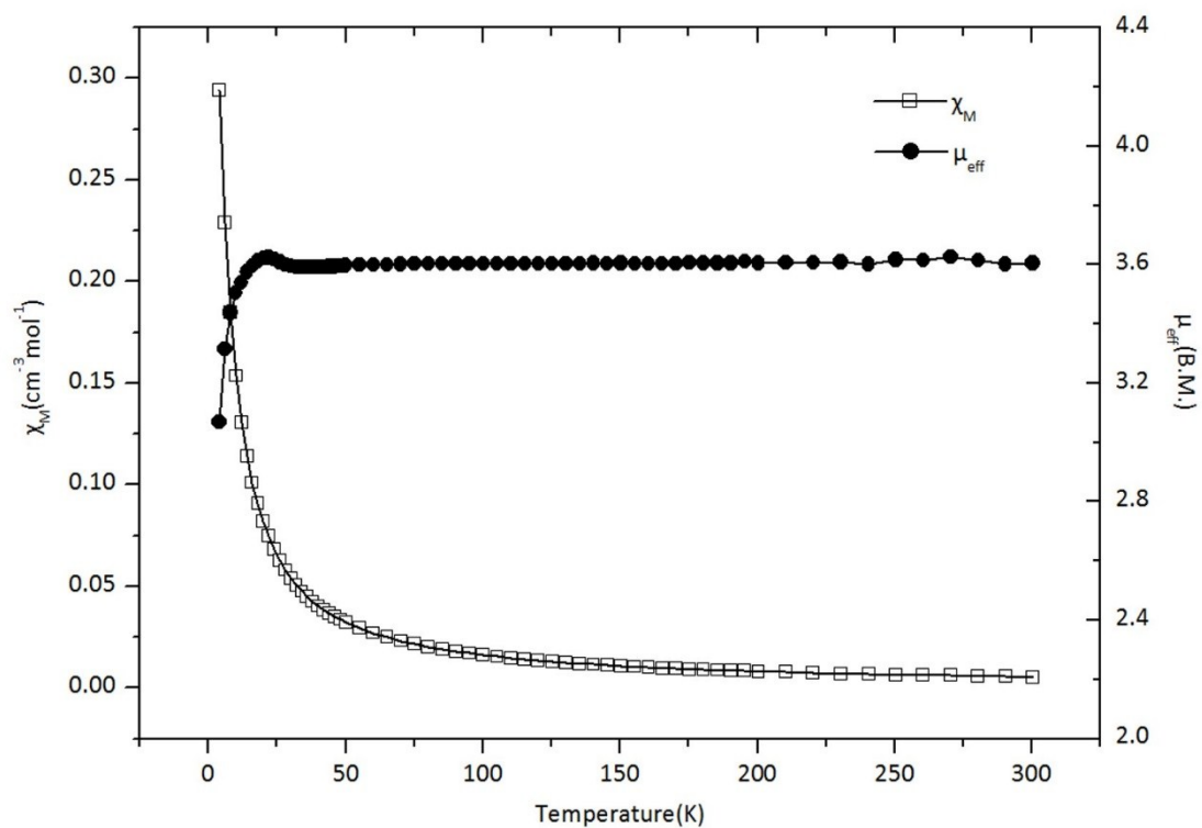
Figure S1. Plots of \chi_M ( \square ) and \mu_{\text{eff}} ( \bullet ) vs. T for 2 . The solid line corresponds to the theoretical fit.
