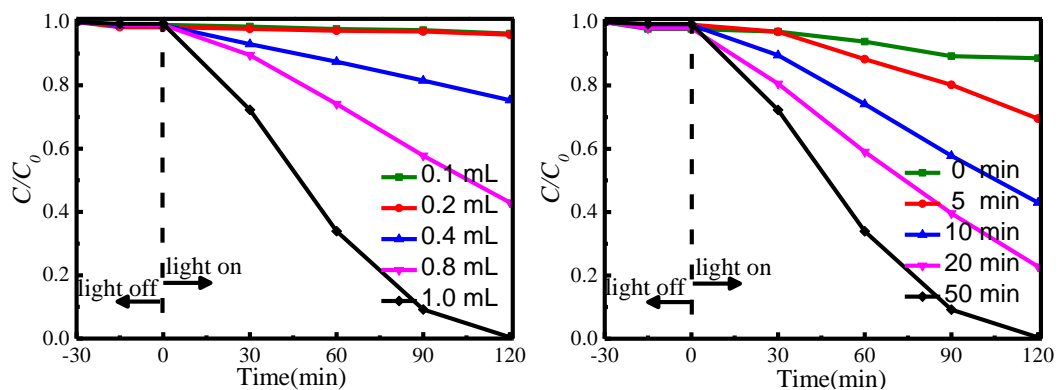
Fig. S2 Photocatalytic activities of as-prepared samples with different reaction conditions: (a) different ammonia addition, and (b) different steeping time.
