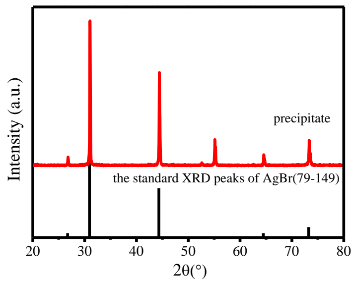
Fig. S3 XRD of samples which produced when \text{AgNO}_3 was added into the supernatant of water-steeping process
