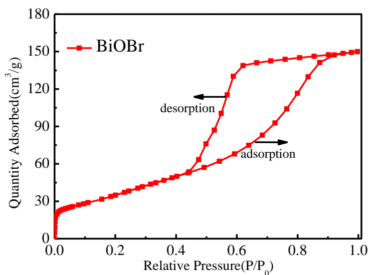
Fig. S1 Nitrogen absorption-desorption isotherms of BiOBr.
