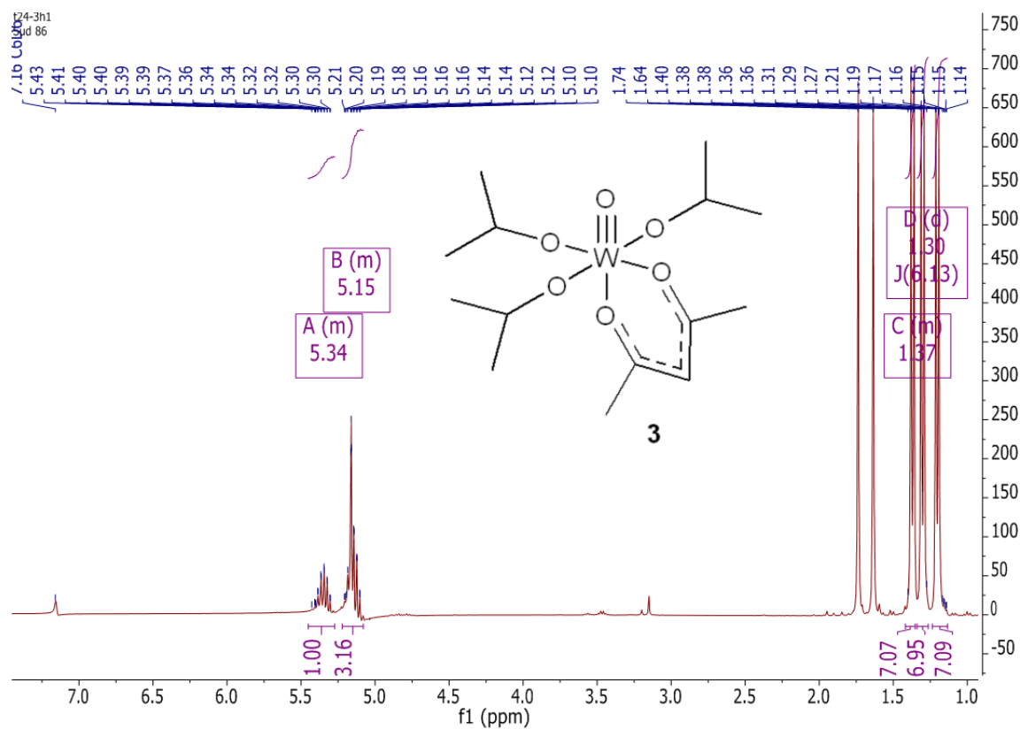
Figure S5: Room temperature 1 H NMR of 3 in C 6 D 6 .
