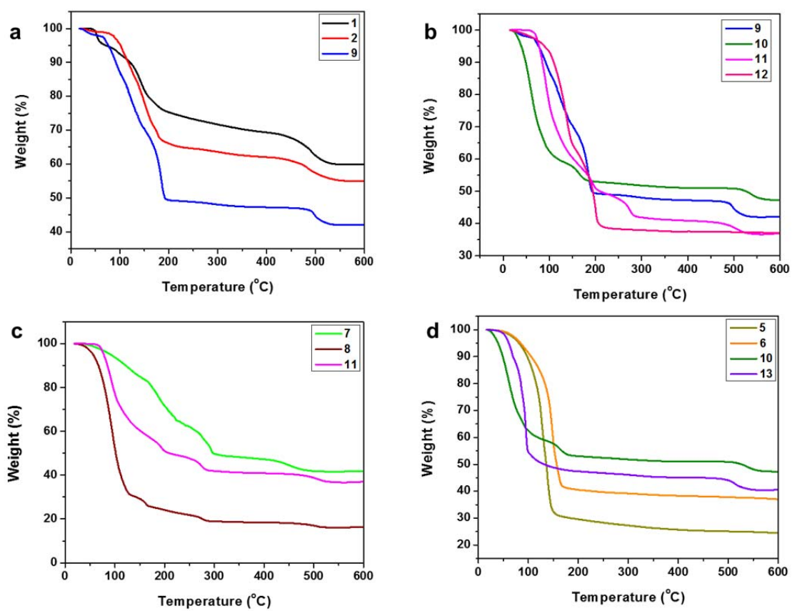
Figure S29. TGA of complexes \text{WO}(\text{OR})_3\text{L} ; a) 1, 2, 9, b) 9, 10, 11, 12, c) 7, 8, 11 and d) 5, 6, 10, 13.
