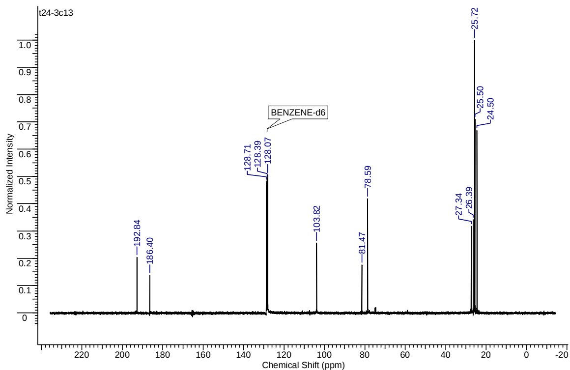
Figure S6: Room temperature 13 C NMR of 3 in C 6 D 6 .
