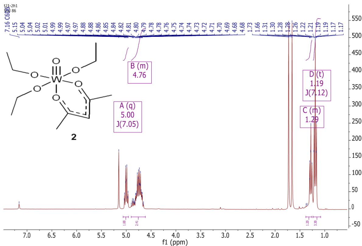
Figure S3: Room temperature 1 H NMR of 2 in C 6 D 6 .
