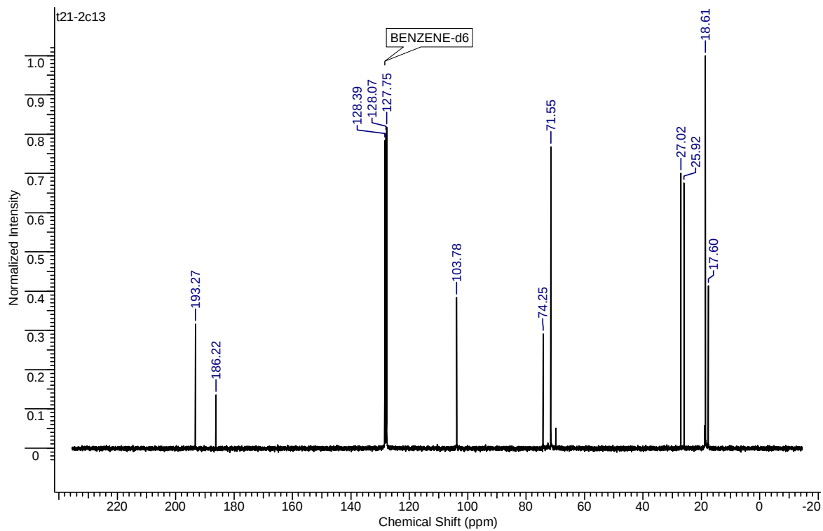
Figure S4: Room temperature 13 C NMR of 2 in C 6 D 6 .
