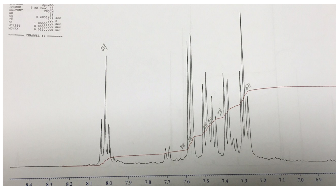
Figure 2: ^1\text{H} NMR Spectrum of [\text{ZnL}][\text{ClO}_4]_2 in aromatic region
