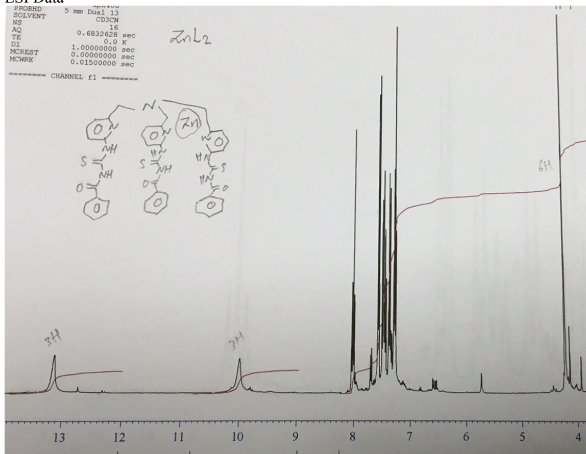
Figure 1:. ^1\text{H} NMR Spectrum of [\text{ZnL}][\text{ClO}_4]
