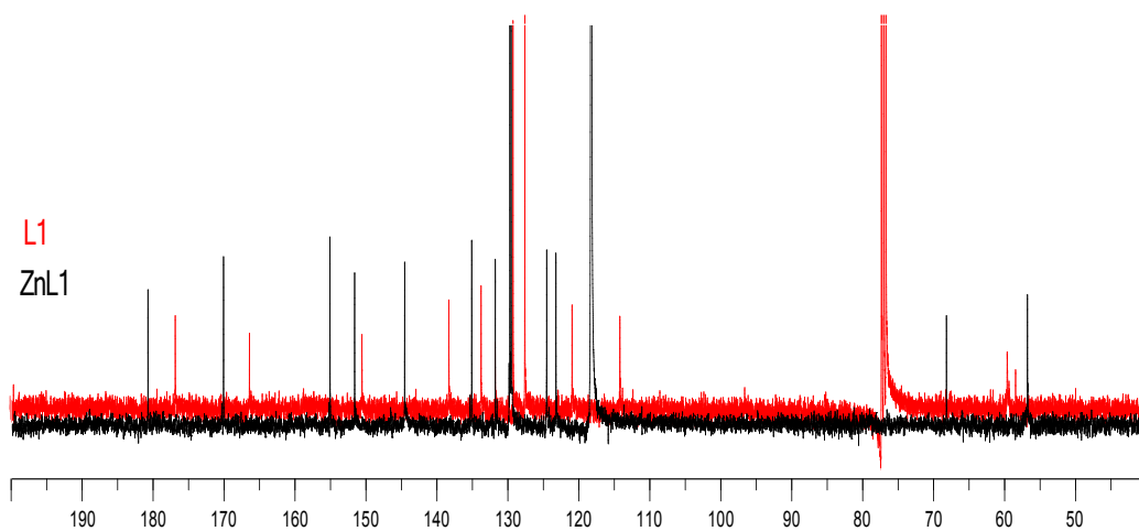
Figure 3: Superimposed ^{13}\text{C} NMR spectra of both the \text{L}^1 (red) and zinc complex (black) of \text{L}^1 .
