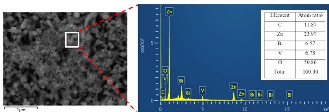
Fig.S1 EDS of the obtained ZnO NRs/BiVO 4
