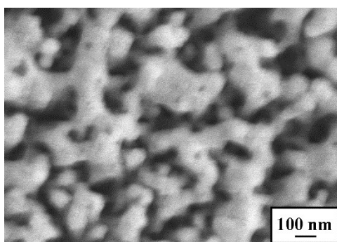
Fig.S3 Top-view SEM images of ZnO NRs/BiVO 4 after 1000s stability testing
