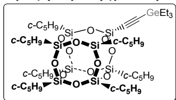
1-((triethylgermyl)ethynyl)-3,5,7,9,11,13,15-hepta(cyclopentyl)pentacyclo[9.5.1.1 3,9 .1 5,15 .1 7,13 ]octasiloxane (4)
