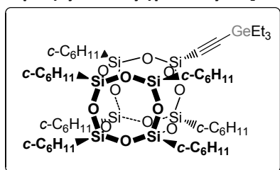
1-((triethylgermyl)ethynyl)-3,5,7,9,11,13,15-hepta(cyclohexyl)pentacyclo[9.5.1.1 3,9 .1 5,15 .1 7,13 ]octasiloxane (6)
