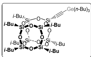
1-((tri( n -butyl)germyl)ethynyl)-3,5,7,9,11,13,15-hepta(isobutyl)pentacyclo[9.5.1.1 3,9 .1 5,15 .1 7,13 ]octasiloxane (2)
