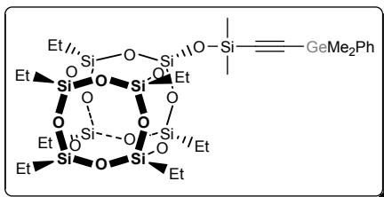
1-((dimethylphenylgermylethynyl)dimethylsiloxy)-3,5,7,9,11,13,15-hepta(ethyl)pentacyclo[9.5.1.1 3,9 .1 5,15 .1 7,13 ]octasiloxane (12)
