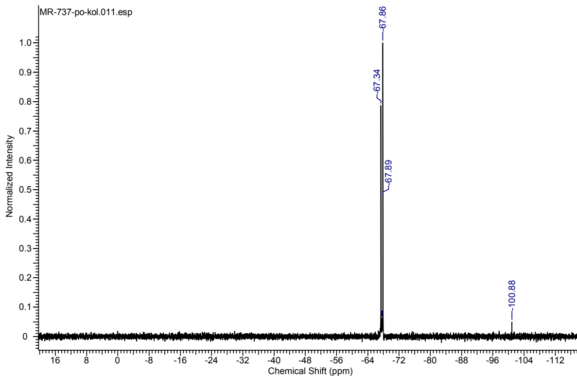
1-((triethylgermyl)ethynyl)-3,5,7,9,11,13,15-hepta(cyclopentyl)pentacyclo[9.5.1.1 3,9 .1 5,15 .1 7,13 ]octasiloxane (4)
