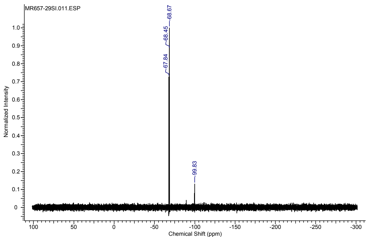
1-((triethylgermylethynyl)dimethylsiloxy)-3,5,7,9,11,13,15-hepta(isobutyl)pentacyclo[9.5.1.1 3,9 .1 5,15 .1 7,13 ]octasiloxane (8)
