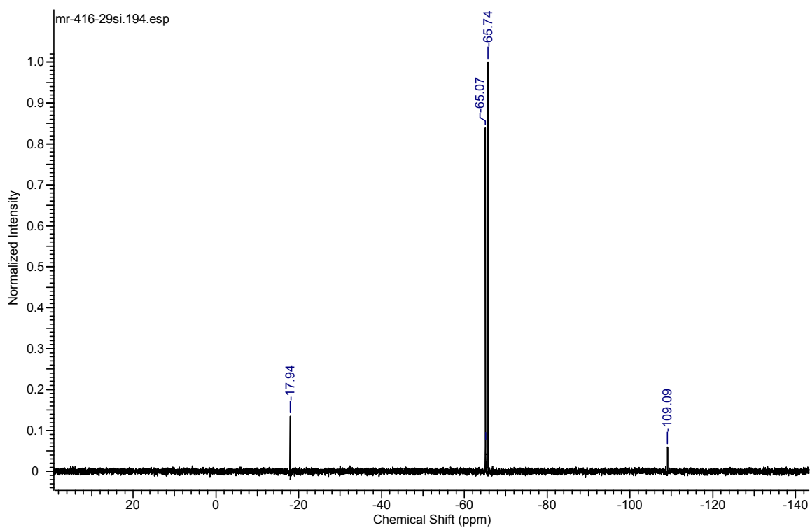
1-((dimethylphenylgermylethynyl)dimethylsiloxy)-3,5,7,9,11,13,15-hepta(ethyl)pentacyclo[9.5.1.1 3,9 .1 5,15 .1 7,13 ]octasiloxane (12)
