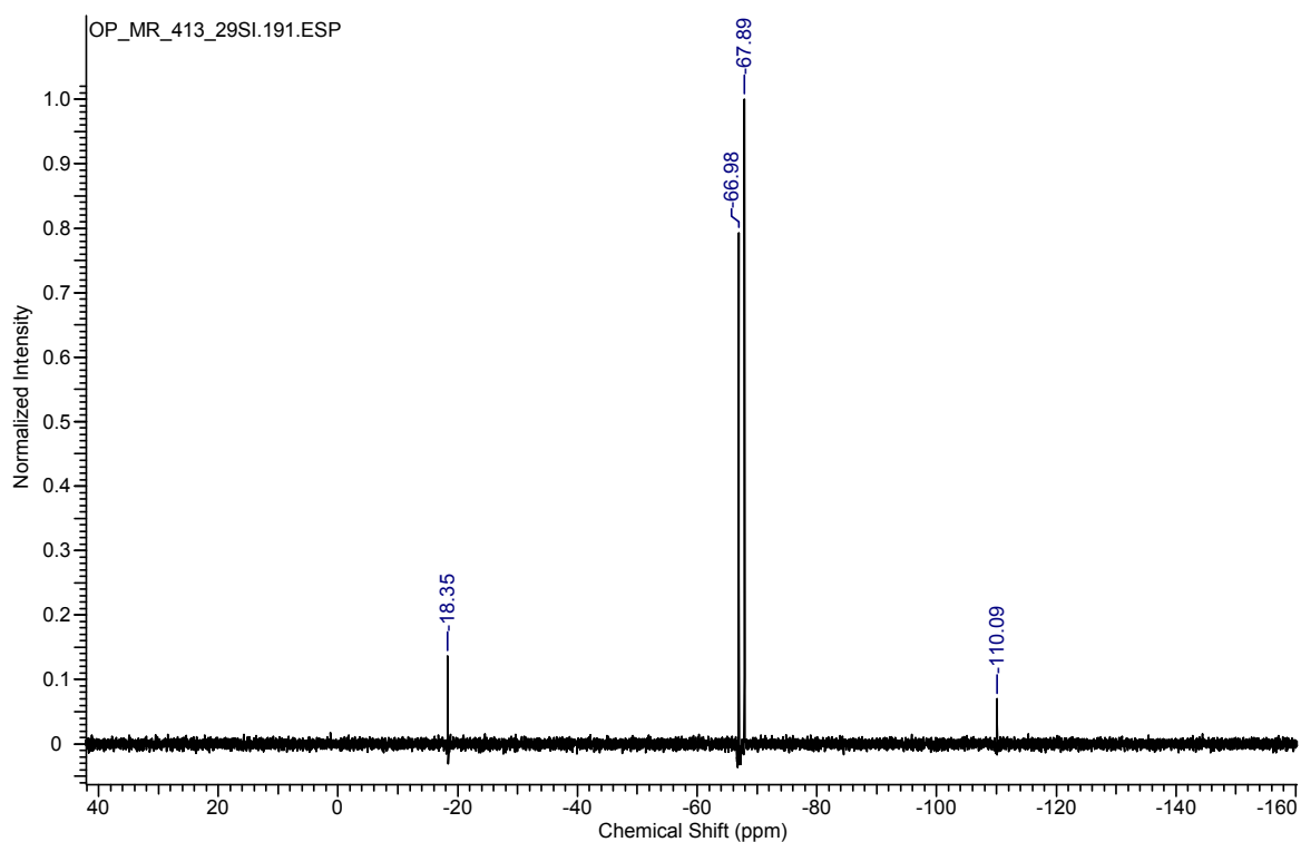
1-((triethylgermylethynyl)dimethylsiloxy)-3,5,7,9,11,13,15-hepta(ethyl)pentacyclo[9.5.1.1 3,9 .1 5,15 .1 7,13 ]octasiloxane (10)
