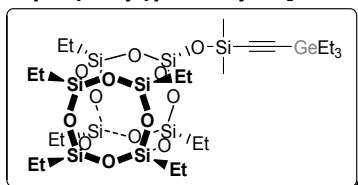
1-((triethylgermylethynyl)dimethylsiloxy)-3,5,7,9,11,13,15-hepta(ethyl)pentacyclo[9.5.1.1 3,9 .1 5,15 .1 7,13 ]octasiloxane (10)
