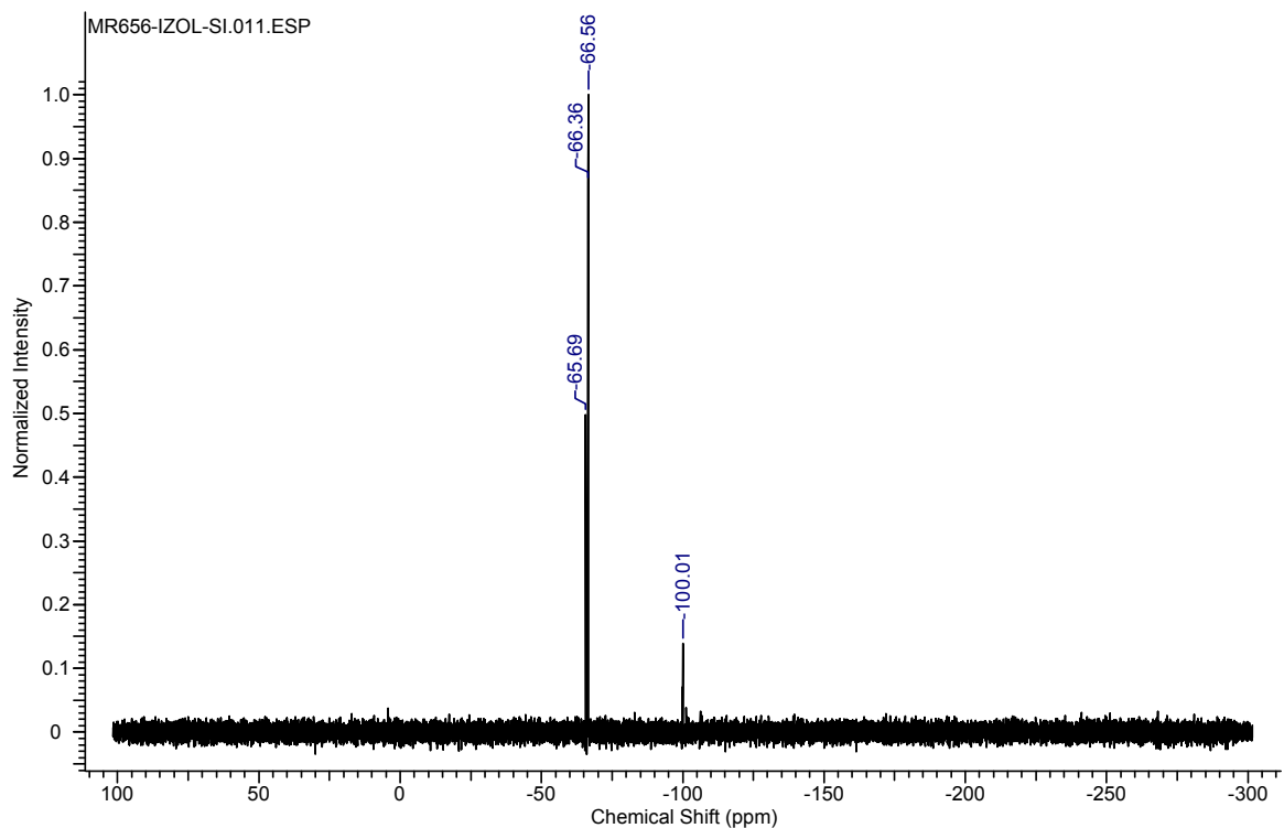
1-((triethylgermyl)ethynyl)-3,5,7,9,11,13,15-hepta(cyclohexyl)pentacyclo[9.5.1.1 3,9 .1 5,15 .1 7,13 ]octasiloxane (6)
