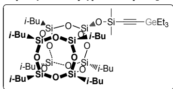
1-((triethylgermylethynyl)dimethylsiloxy)-3,5,7,9,11,13,15-hepta(isobutyl)pentacyclo[9.5.1.1 3,9 .1 5,15 .1 7,13 ]octasiloxane (8)
