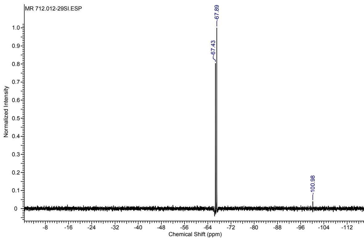
1-((tri( n -butyl)germyl)ethynyl)-3,5,7,9,11,13,15-hepta(isobutyl)pentacyclo[9.5.1.1 3,9 .1 5,15 .1 7,13 ]octasiloxane (2)
