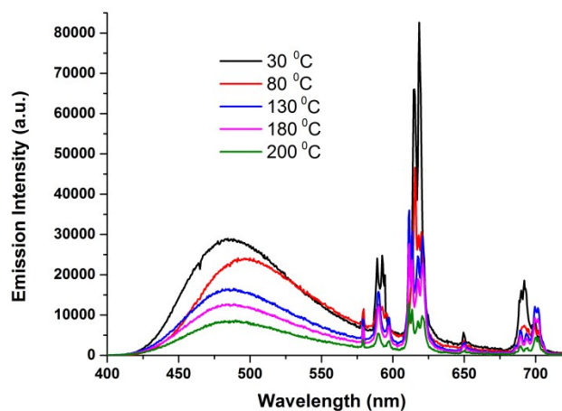
Fig. S4 Temperature-dependent emission spectrum of complex 2 upon excitation at 380nm.
