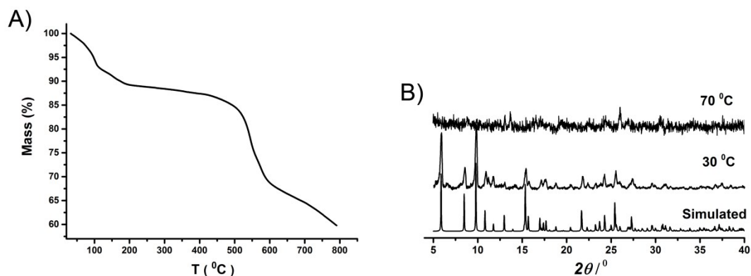
Fig. S1 Thermogravimetric analysis (A) and temperature-dependent PXRD measurement (B) for complex 1 .
