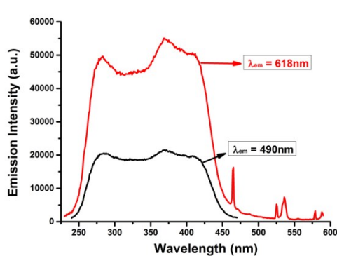
Fig. S2 Excitation spectrum of complex 2 .
