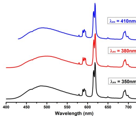
Fig. S3 Emission spectrum of complex 2 under excitation of near-UV light.
