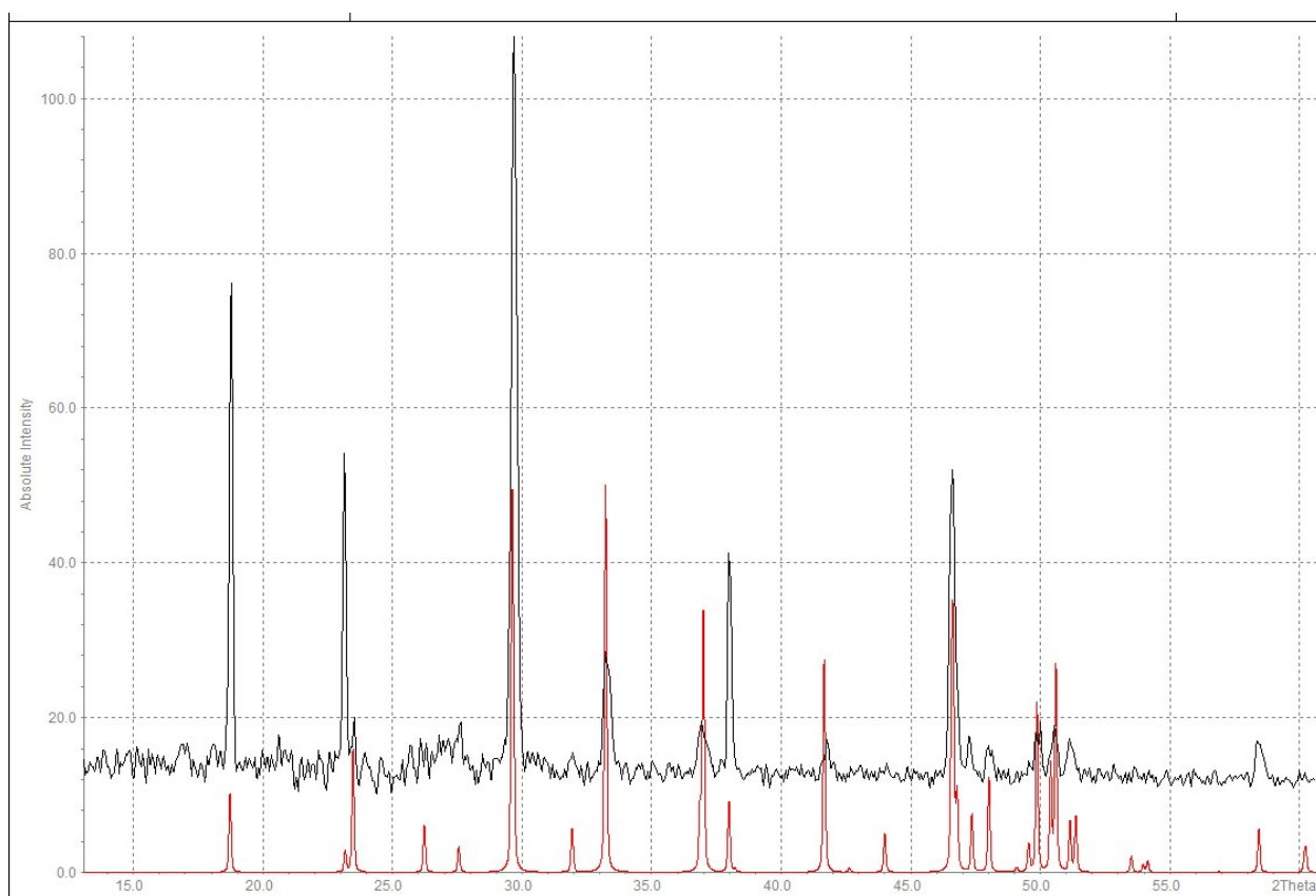
Diffraction pattern of a polycrystalline sample NO[BF 4 ] (shown in black) in comparison with the theoretical curve (red).
