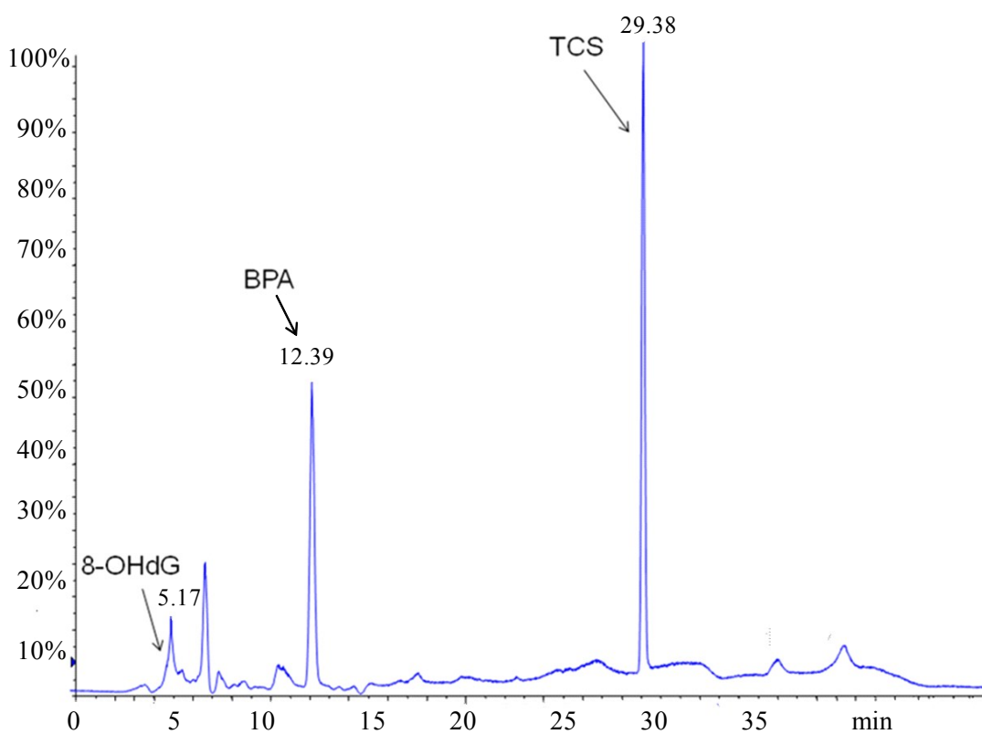
Fig 2: The chromatogram of urinary 8-OHdG, TCS and BPA in a real urine sample
