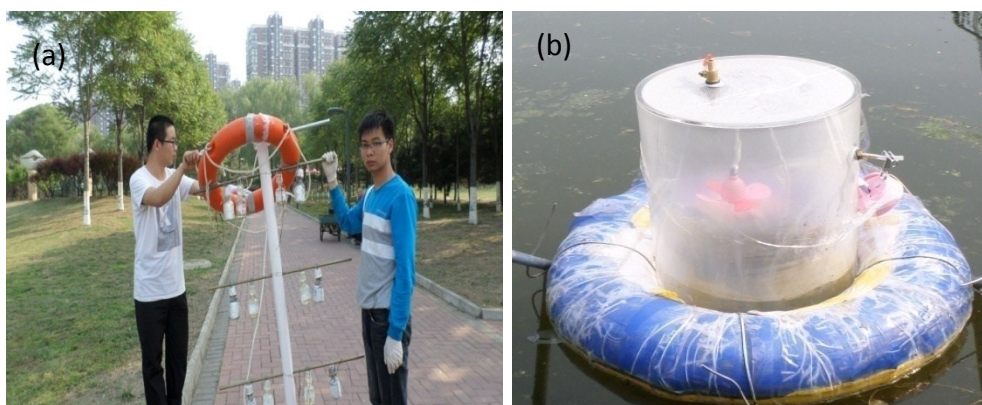
Fig. S1 The sampling device figure of photosynthesis (a) and water-air CO 2 exchange (b)
