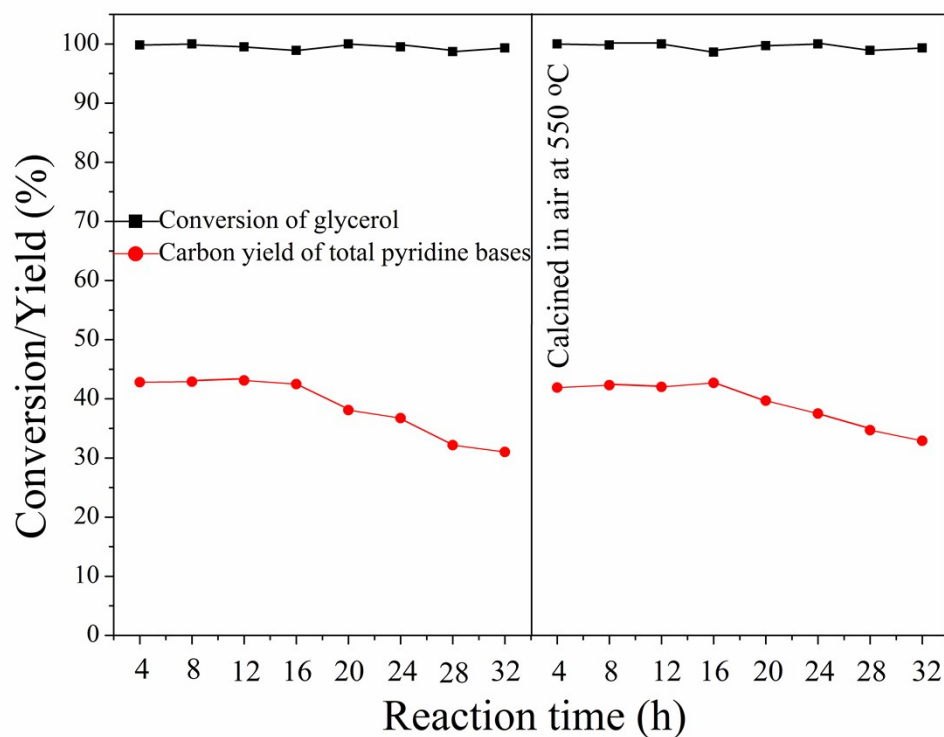
Fig. S1 Glycerol conversion and total yield of pyridine bases as functions of reaction time.
