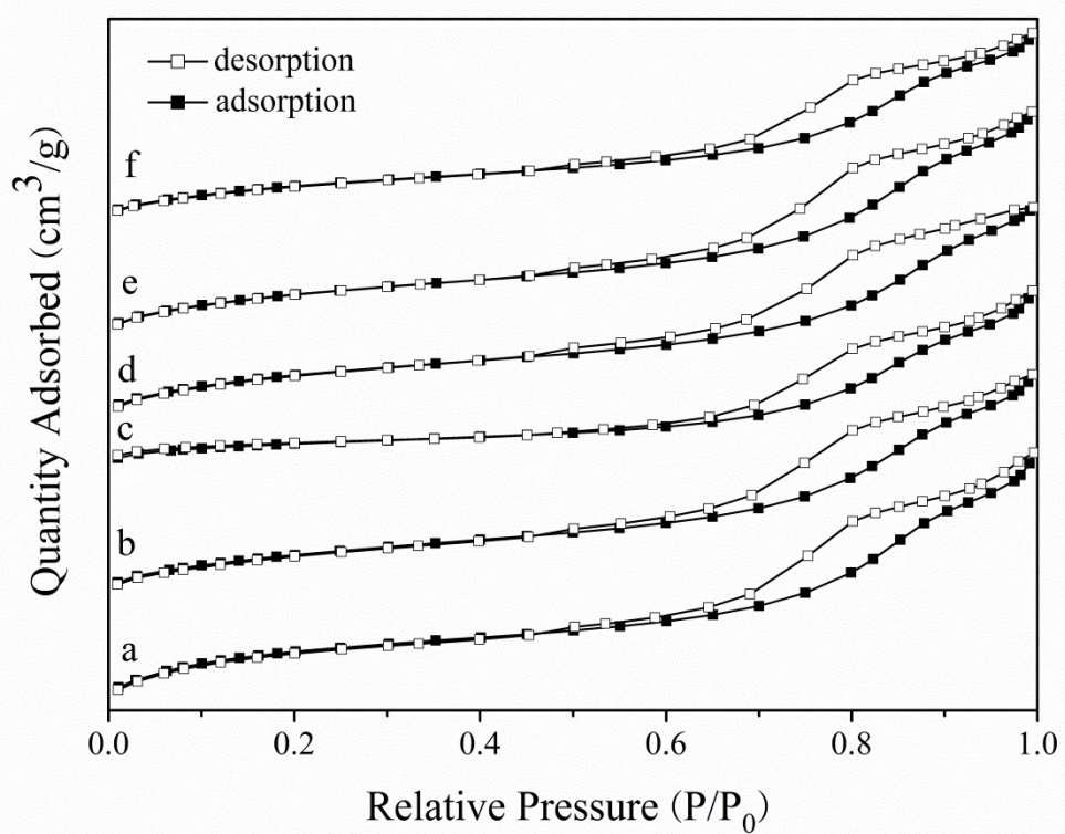
Fig. S2 Adsorption–desorption isotherms of the catalyst samples. (a) HZSM-5(38); (b) 4.6%Cu/HZSM-5(38) (Fresh); (c) 4.6%Cu/HZSM-5(38) (Used); (d) 4.6%Cu/HZSM-5(38) (Regenerated); (e) 2.3%Cu/HZSM-5(38); (f) 15.3%Cu/HZSM-5(38).
