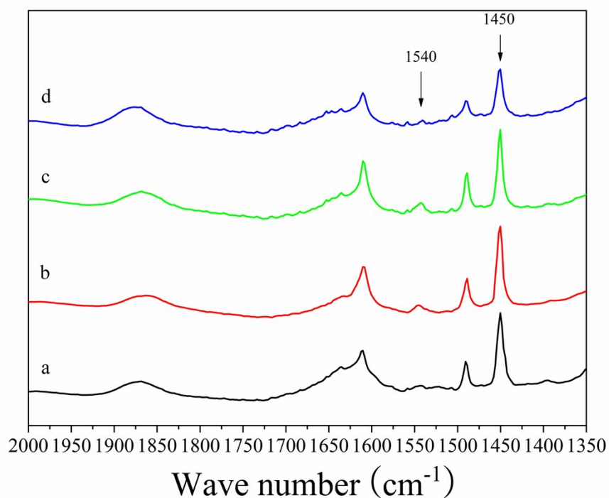
Fig. S5 (2) IR spectra of pyridine adsorbed on the catalysts. (a) 2.3%Cu/HZSM-5(25); (b) 2.3%Cu/HZSM-5(38); (c) 2.3%Cu/HZSM-5(80); (d) 2.3%Cu/HZSM-5(117).
