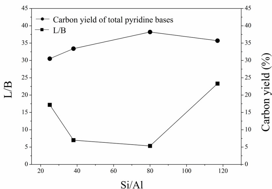
Fig. S5 (1) Effects of the Si/Al ratio on the L/B ratio and the performance of the 2.3%Cu/HZSM-5 catalysts.
