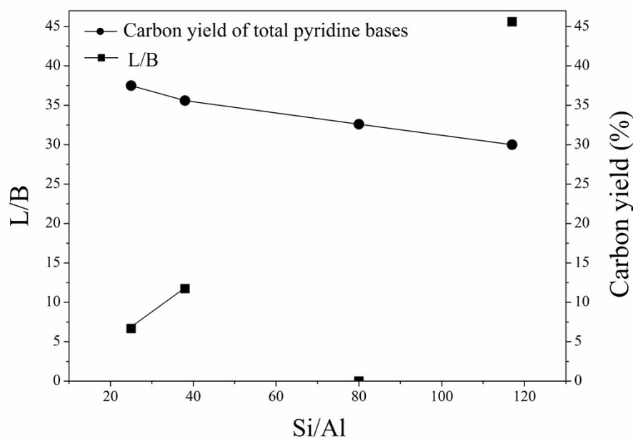
Fig. S6 (1) Effects of the Si/Al ratio on the L/B ratio and the performance of the 6.9%Cu/HZSM-5 catalysts.
