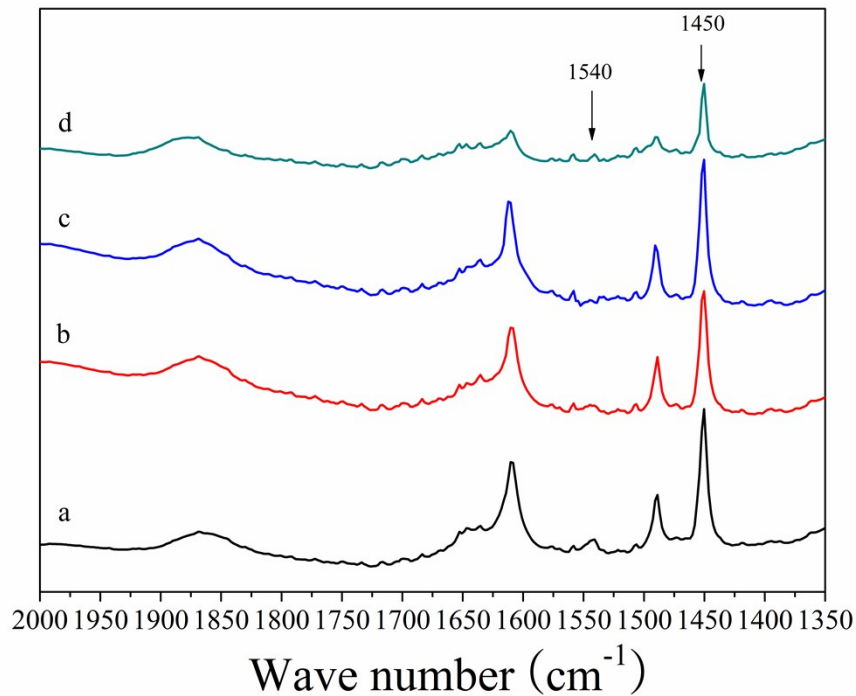
Fig. S6 (2) IR spectra of pyridine adsorbed on the catalysts. (a) 6.9%Cu/HZSM-5(25); (b) 6.9%Cu/HZSM-5(38); (c) 6.9%Cu/HZSM-5(80); (d) 6.9%Cu/HZSM-5(117).
