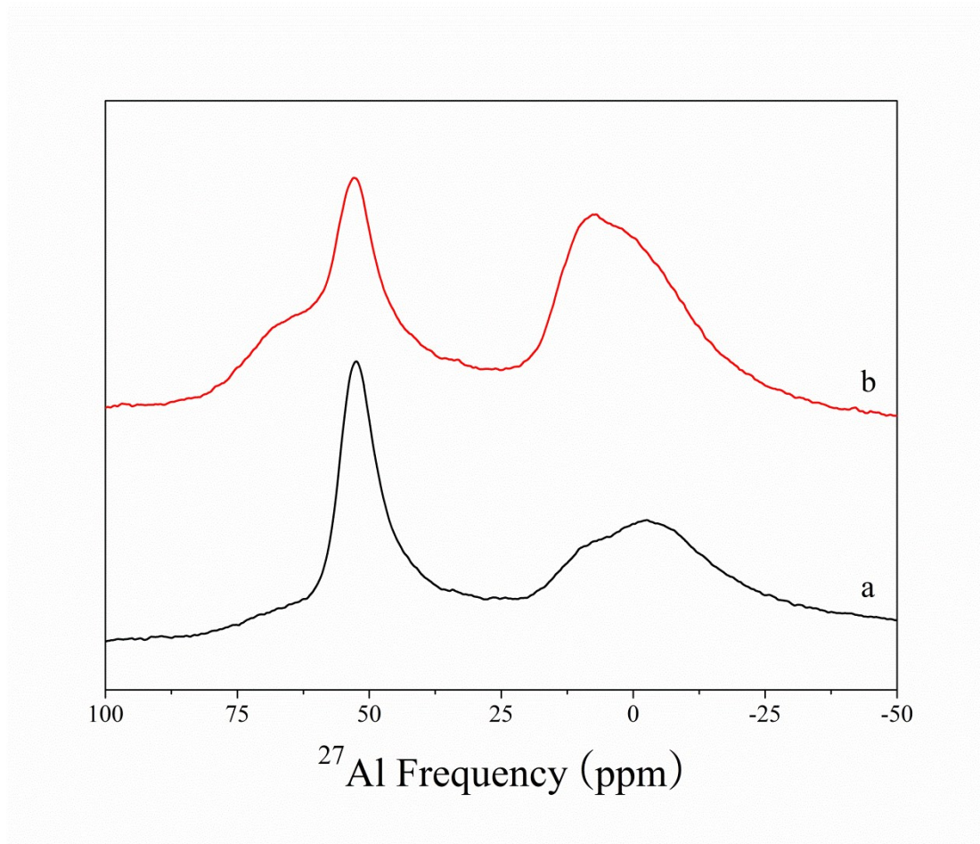
Fig. S8 ^{27}\text{Al} -MAS-NMR spectra of the Cu/HZSM-5 zeolites samples. (a) 4.6%Cu/HZSM-5(38) (Fresh); (b) 4.6%Cu/HZSM-5(38) (Regenerated).
