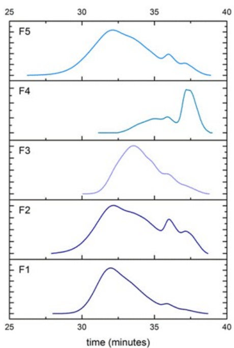
Fig. S1 – Gel permeation chromatograms of acetylated solid residues isolated from F1-F5.
