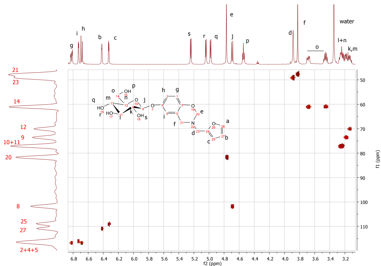
Fig. S1. 1 H- 13 C HSQC spectrum of A-Fa. DMSO d 6 .
