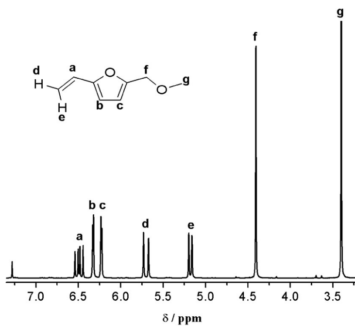
Figure S5. 1 H NMR spectrum of MMVF (in CDCl 3 , 300 MHz).
