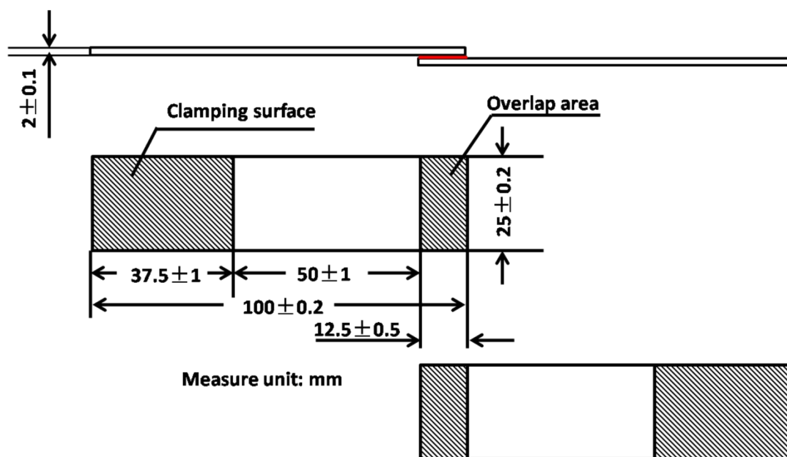
Figure S3. Schematic of the sandwiched sample for the lap shear test.
