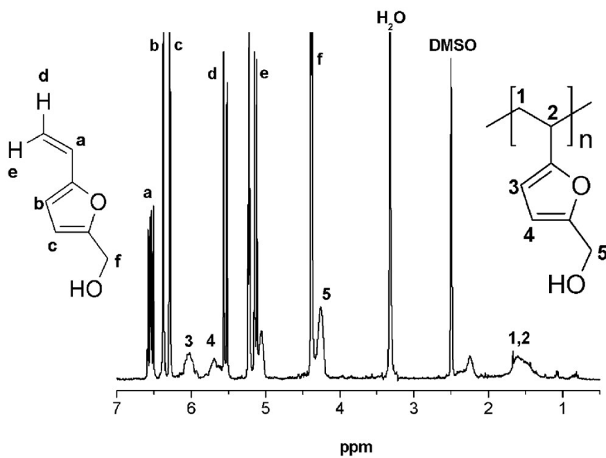
Figure S7. ^1\text{H} NMR spectrum of PHMVf (in \text{DMSO} , 400 MHz).
