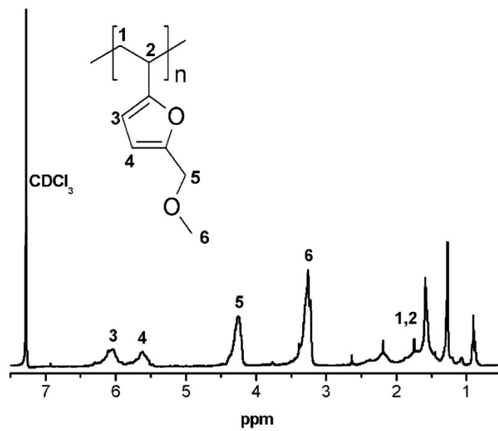
Figure S6. ^1\text{H} NMR spectrum of PMMVF (in \text{CDCl}_3 , 300 MHz).
