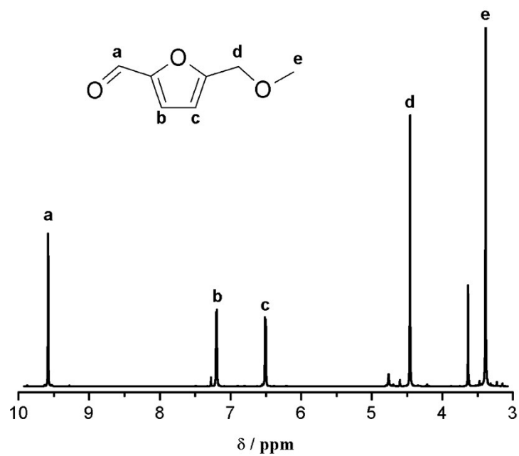
Figure S4. 1 H NMR spectrum of MMF (in CDCl 3 , 300 MHz).
