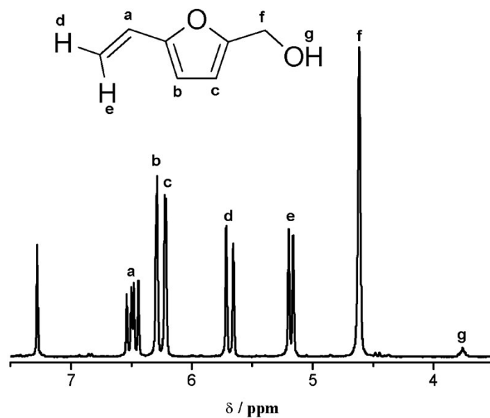
Figure S2. ^1\text{H} NMR spectrum of the HMVF (in \text{CDCl}_3 , 300 MHz).
