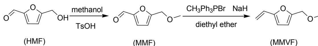
Scheme S1. Synthesis of MMVF.
