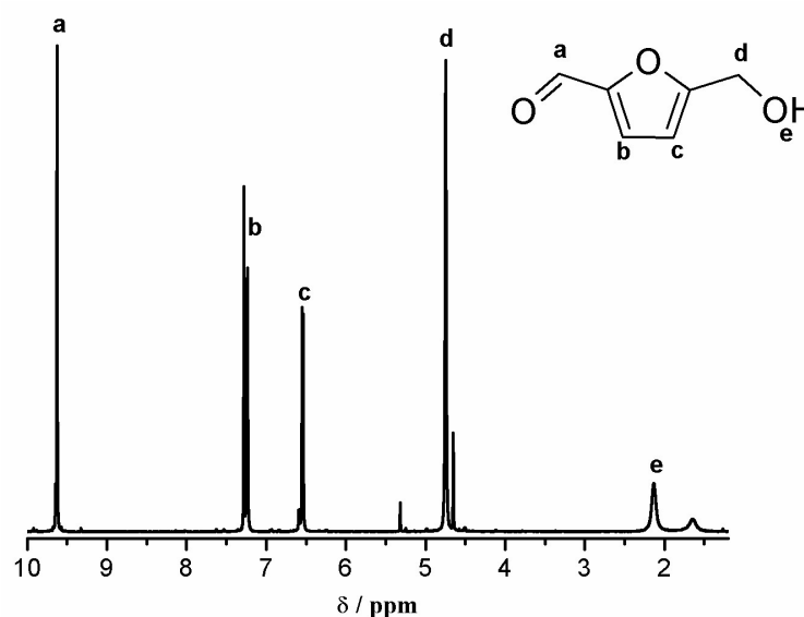
Figure S1. 1 H NMR spectrum of the HMF (in CDCl 3 , 300 MHz).
