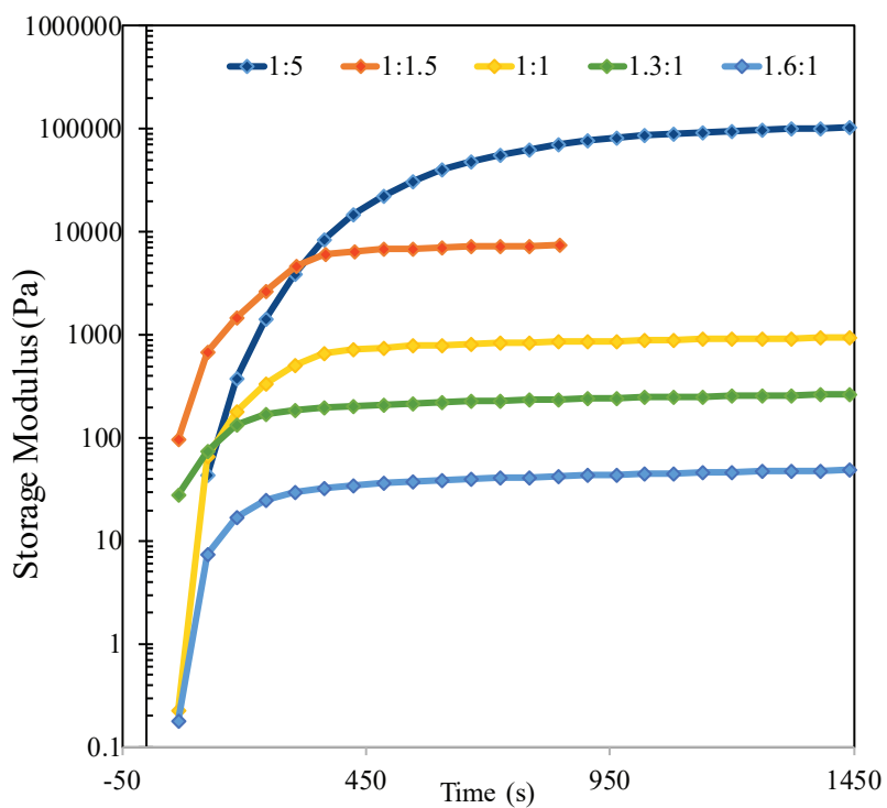
Supplemental Figure 1. Curing test of different monomer to crosslinker ratios at 60°C, with constant shear deformation at frequency of 1Hz. Measurements were taken every 60 seconds.
