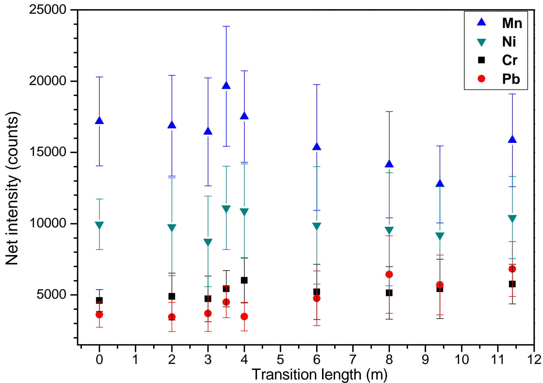
Figure. LIBS net intensities corresponding to the analyzed steel samples of GDU transition (each point, average of 40 shots).
