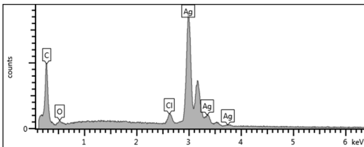
Figure S2. EDS spectrum of Ag/AgCl-coated thread containing Ag, C, Cl and O.
