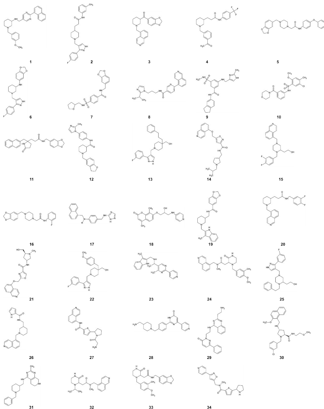
Fig. S1. The structures of the 34 diverse compounds.
