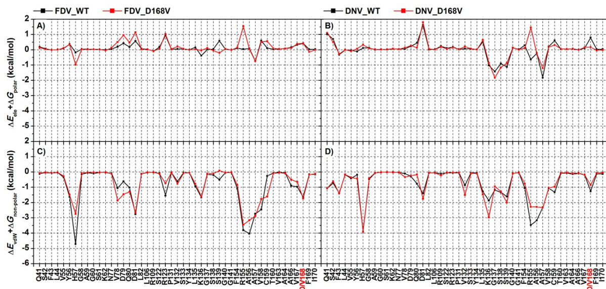
Fig. S1 Energetic components contributed from electrostatic ( \Delta E_{ele} + \Delta G_{polar} ) and van der Waals ( \Delta E_{vdW} + \Delta G_{non-polar} ) terms of NS3 protease domain for wild-type and D168V complexes as shown in black and red lines,
